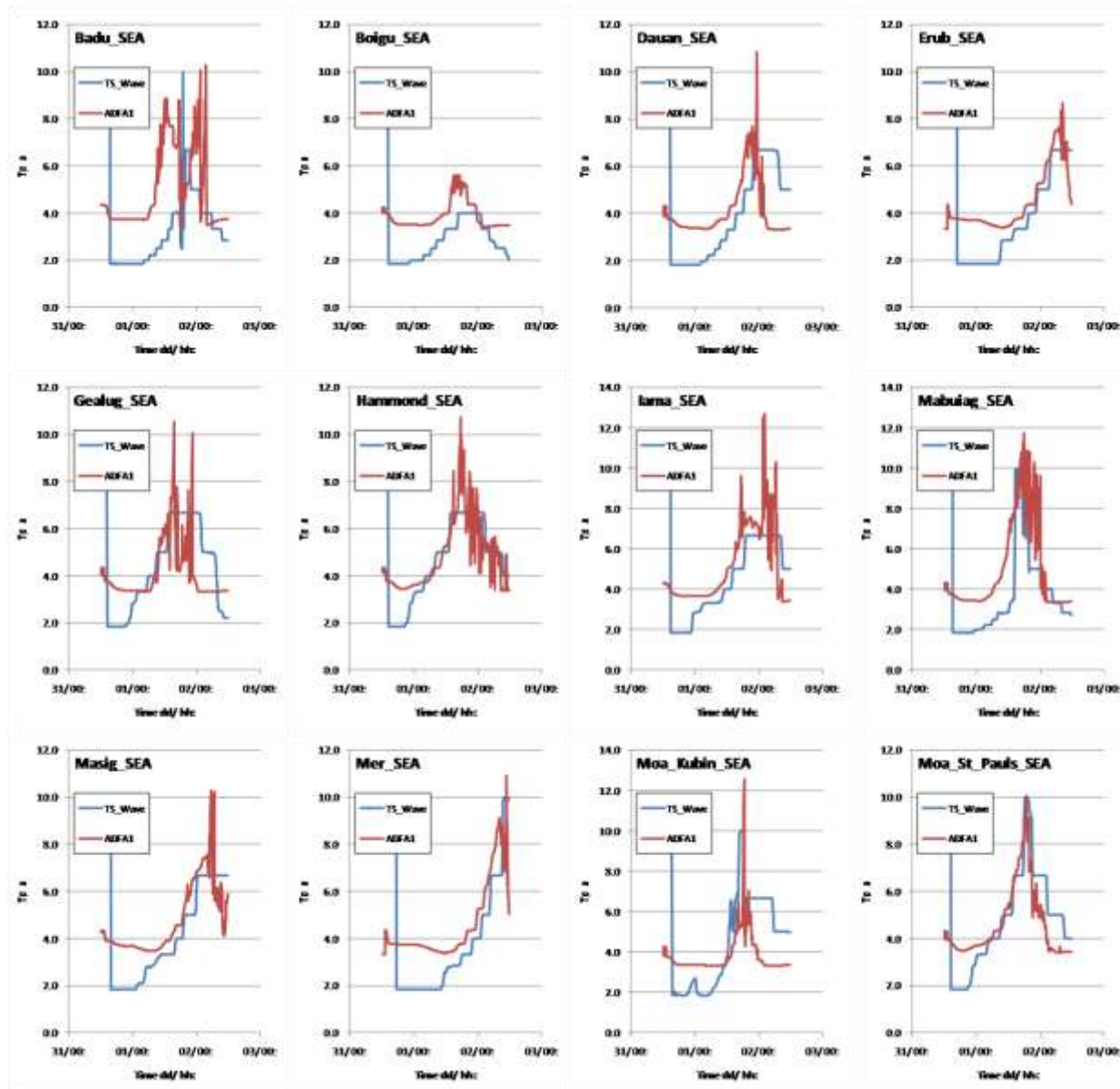
Figure L-1d Example W-E Category 4 TC through Centre (Tp time series comparisons)
