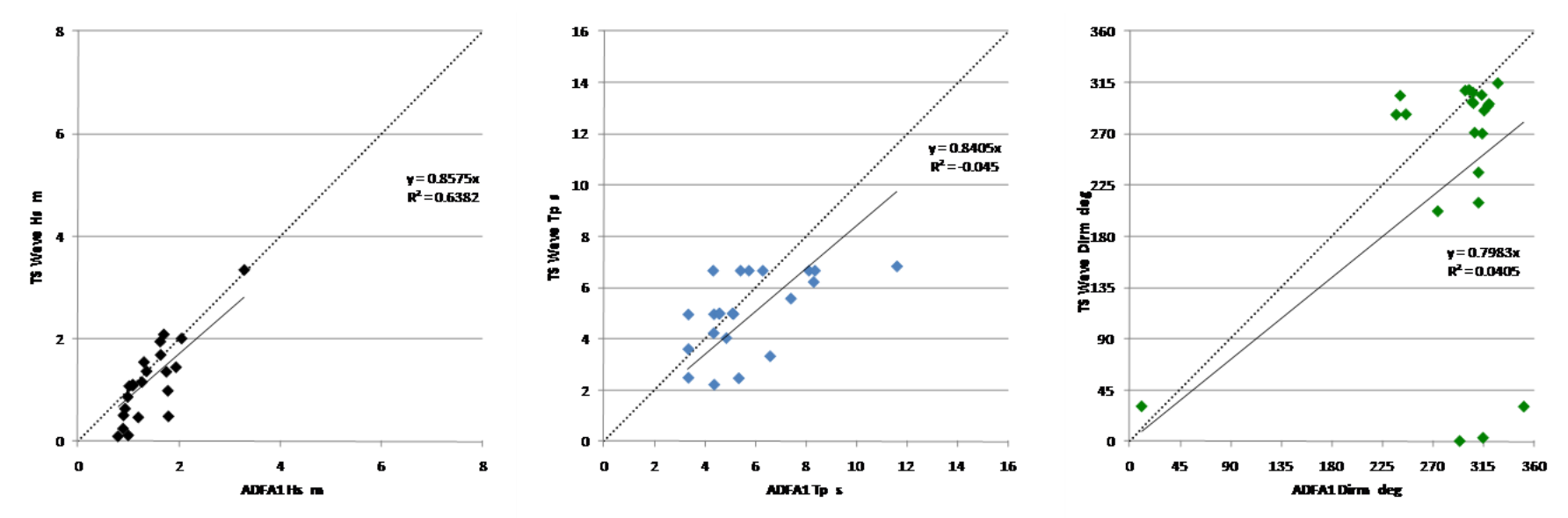
Figure L-4b Example E-W Category 4 TC through Cape York (peak site-specific Hs summary and associated Tp and Mean Direction)
