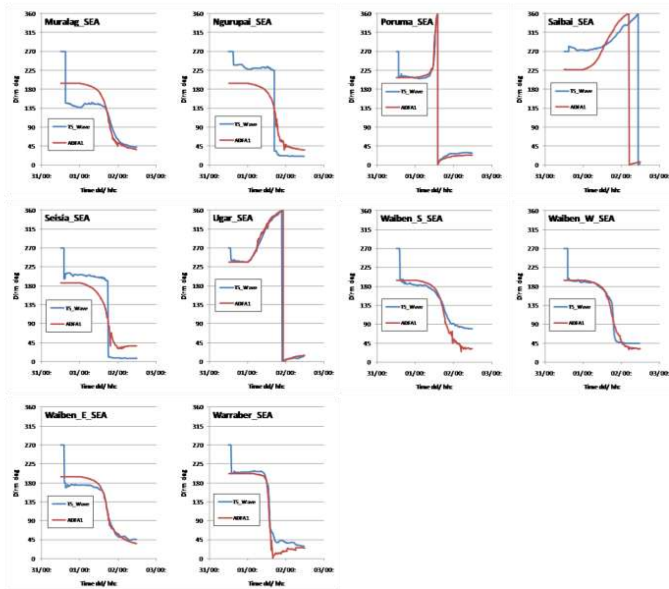
Figure L-3e Example E-W Category 4 TC through Centre (Mean Direction time series comparisons) contd
