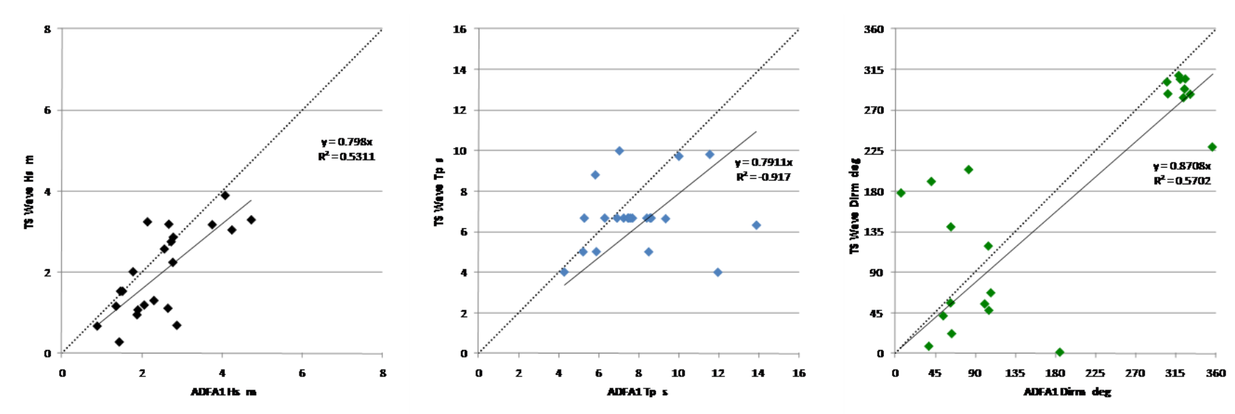
Figure L-3b Example E-W Category 4 TC through Centre (peak site-specific Hs summary and associated Tp and Mean Direction)
