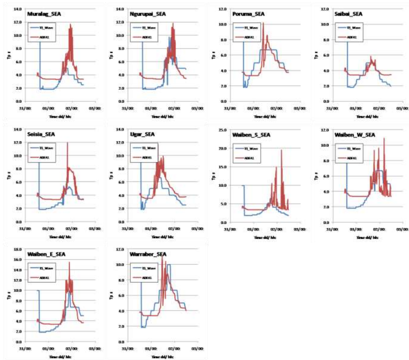
Figure L-3d Example E-W Category 4 TC through Centre (Tp time series comparisons) contd
