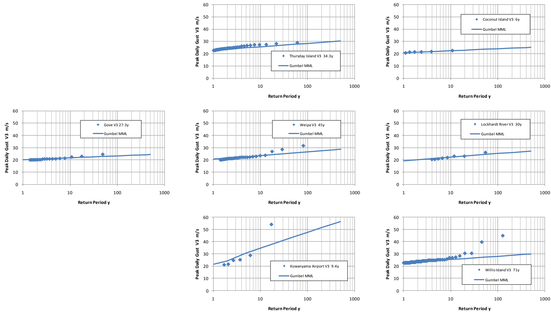
NON-CYCLONIC WIND DATA - PEAK DAILY GUST V3
