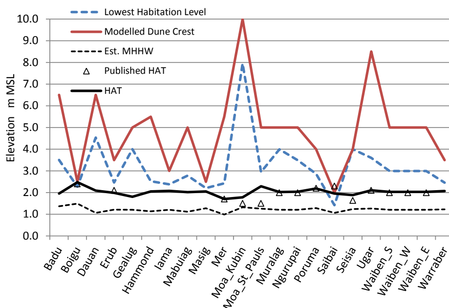
Figure 9-1 Adopted local MSL-relative datums.
