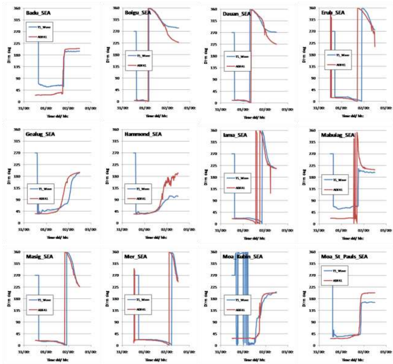
Figure L-1e Example W-E Category 4 TC through Centre (Mean Direction time series comparisons)
