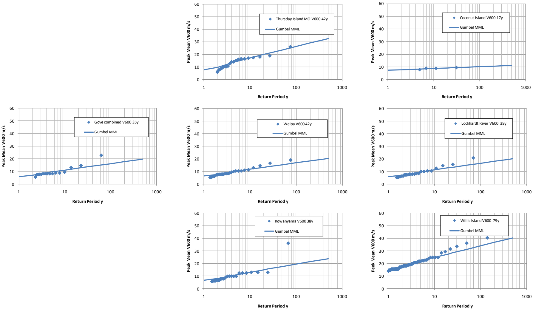
CYCLONIC WIND DATA - MAXIMUM MEAN WINDS V600
