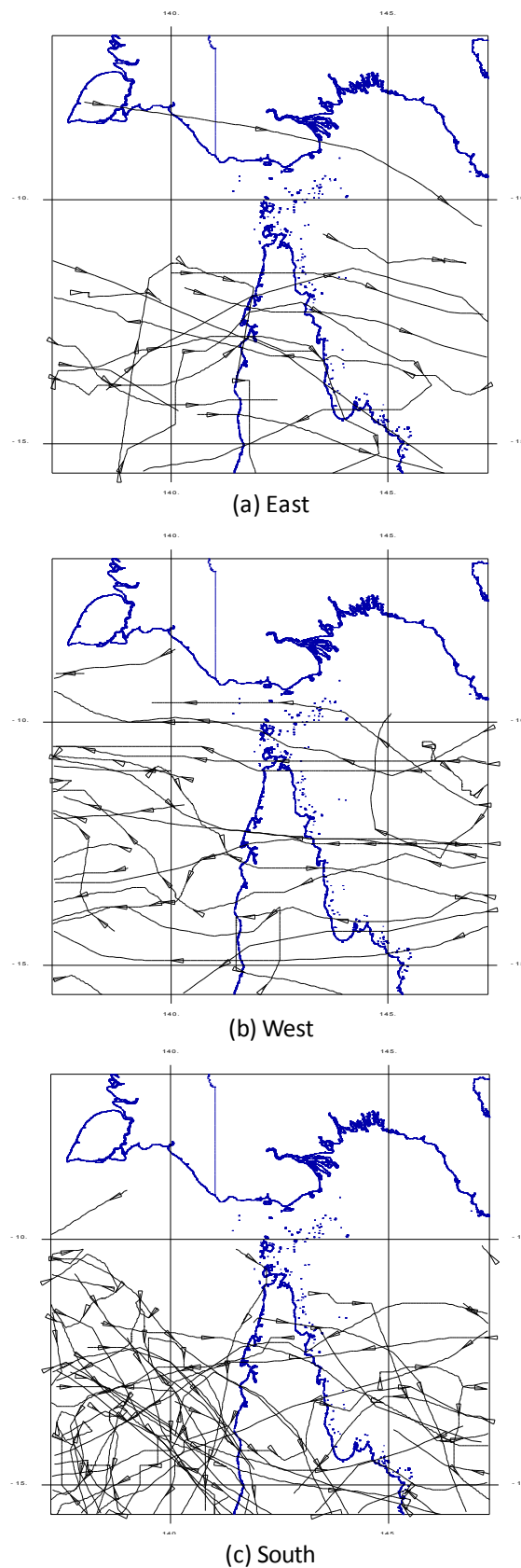
Figure 6-10 Separation of the TC tracks into directional classes.
