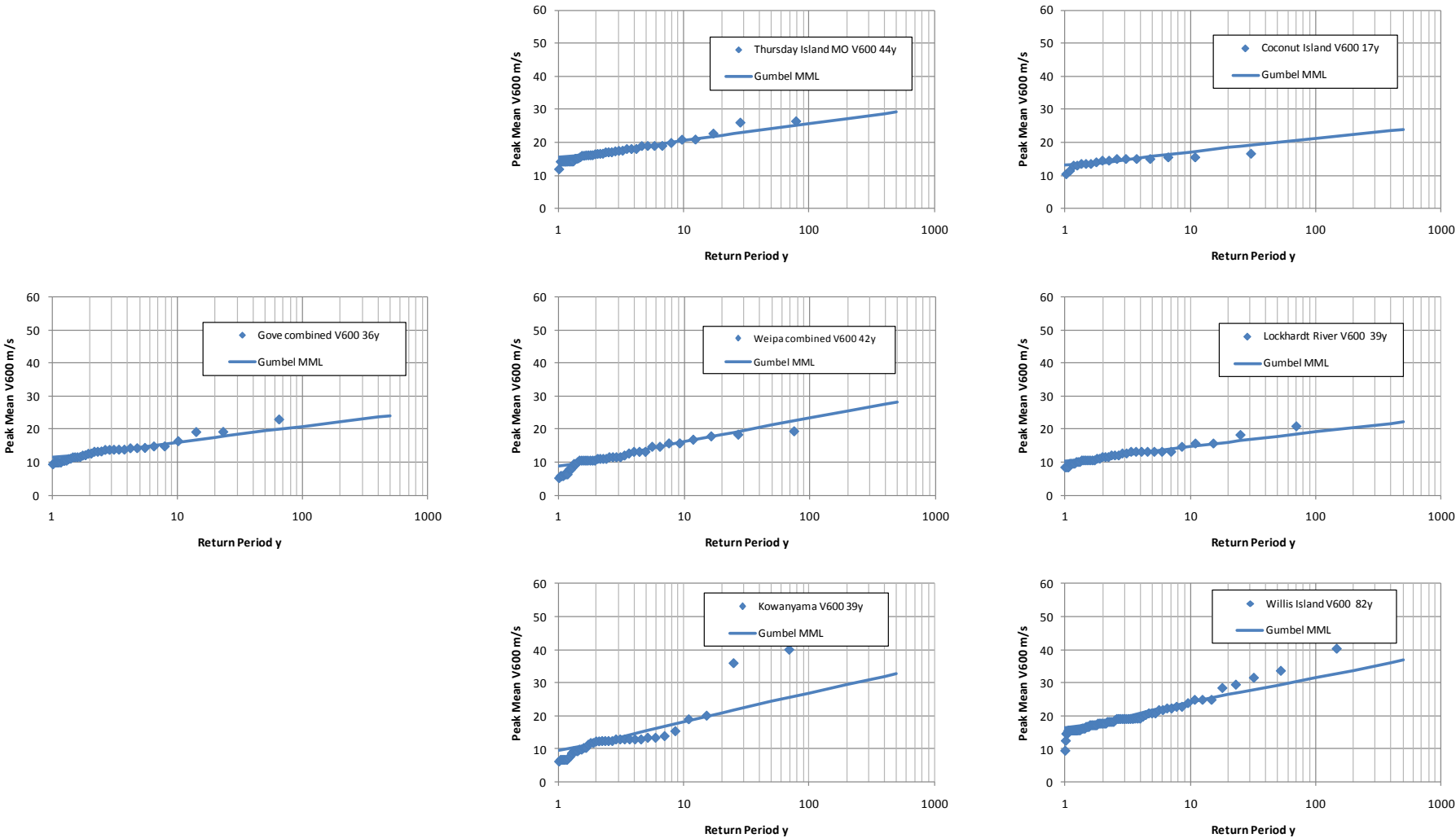
ALL WIND DATA - MAXIMUM MEAN WINDS V600
