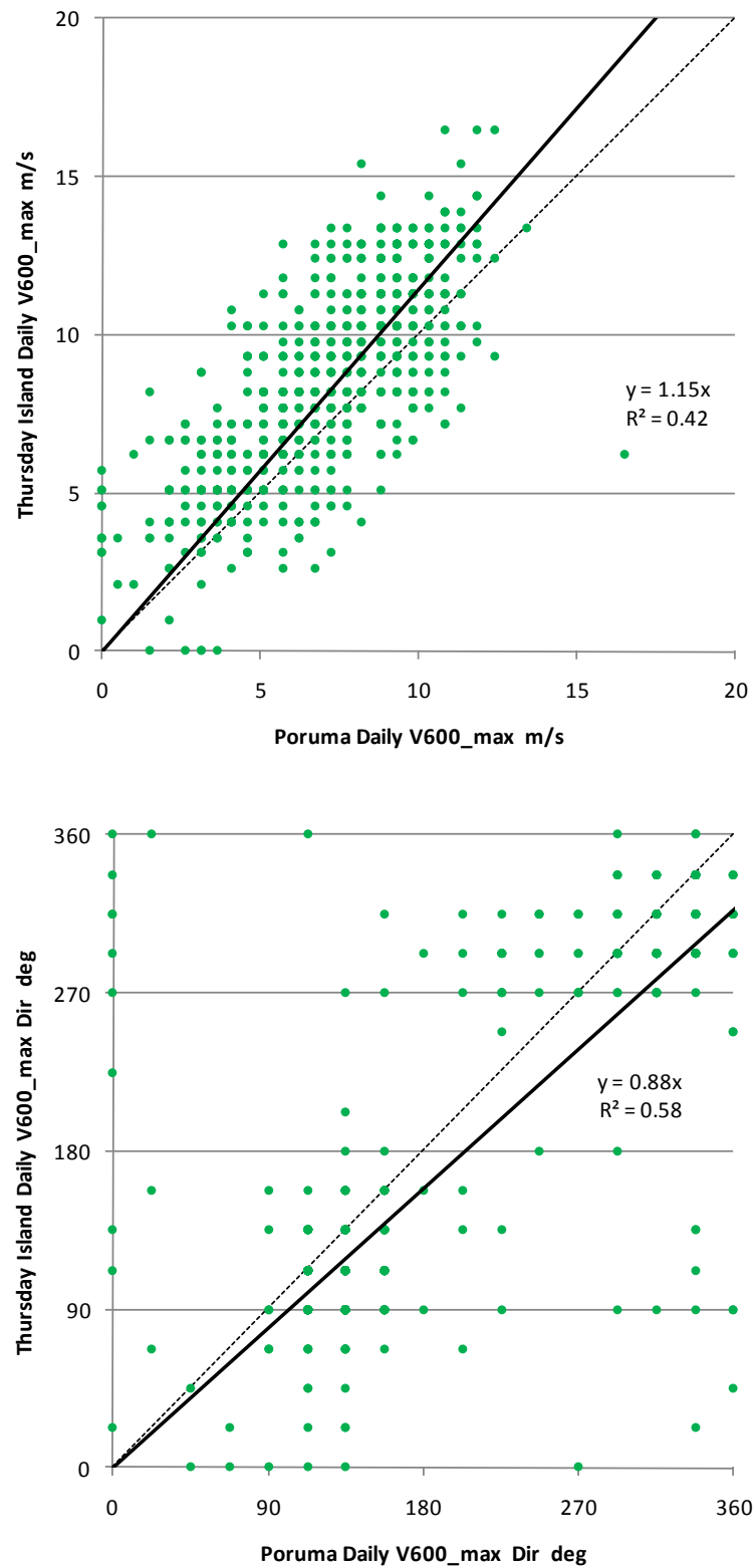
Figure 3-9 Comparison of adjusted Thursday Island and Poruma winds 1994 – 2004.
