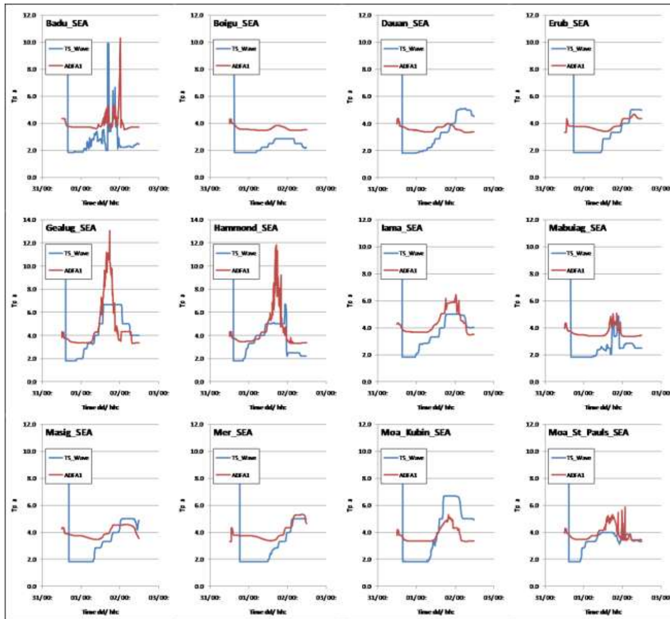
Figure L-2d Example W-E Category 4 TC through Cape York (Tp time series comparisons)
