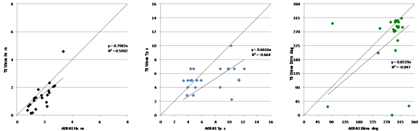
Figure L-2b Example W-E Category 4 TC through Cape York (peak site-specific Hs summary and associated Tp and Mean Direction)
