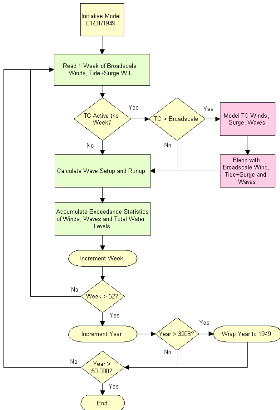
Figure 11-1 Schematic of the operation of the Torres Strait SATSIM model.
