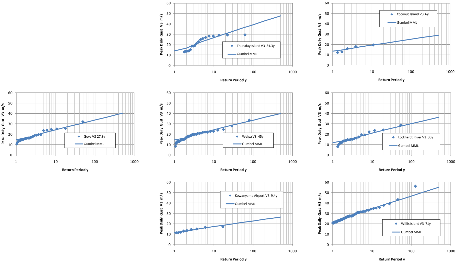
CYCLONIC WIND DATA - PEAK DAILY GUST V3
