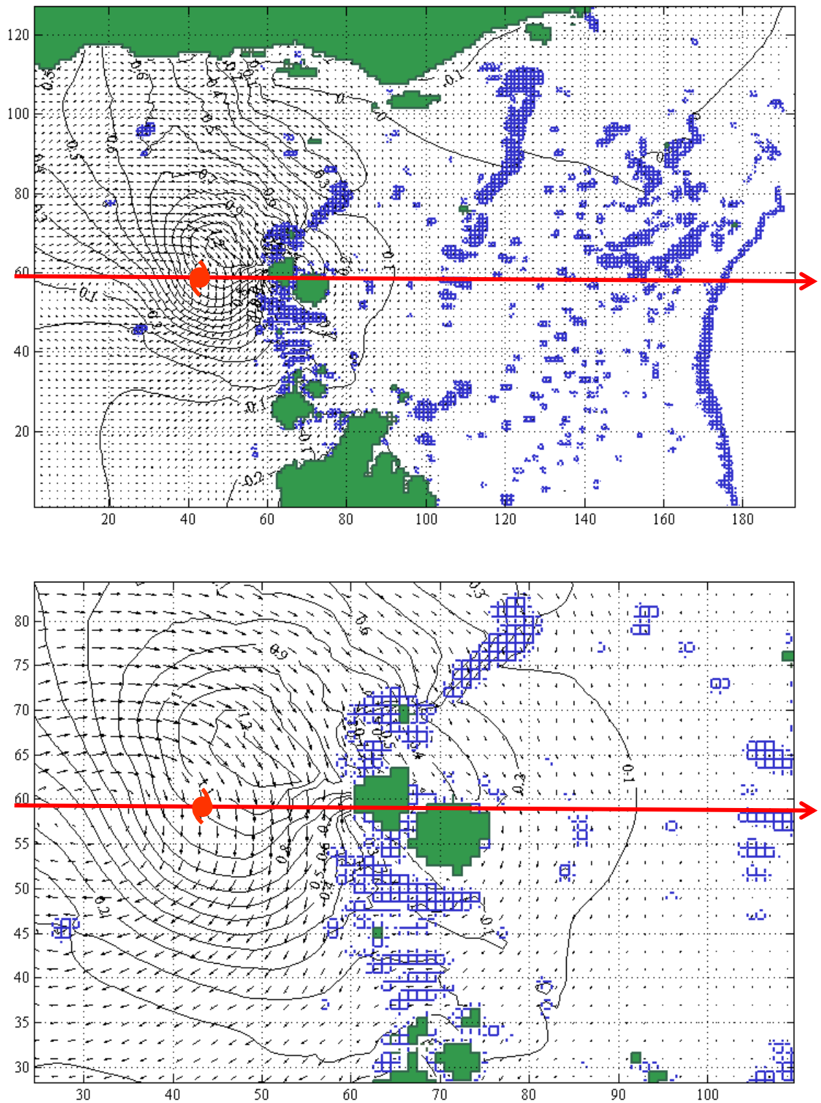
Figure 7-6 Example Cat 4 W-E Centre extreme surge pattern.
