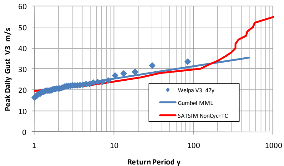
Figure 11-6 SATSIM-simulated wind speeds at Thursday Island for a 50,000 y period compared with the available (adjusted) wind speed record at Weipa.
