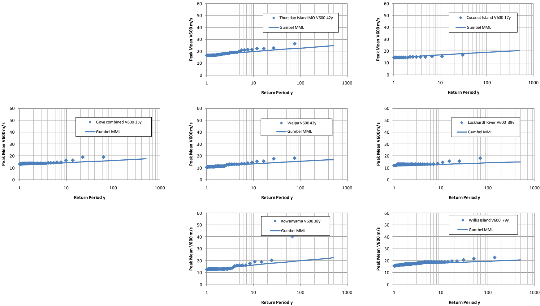
NON-CYCLONIC WIND DATA - MAXIMUM MEAN WINDS V600
