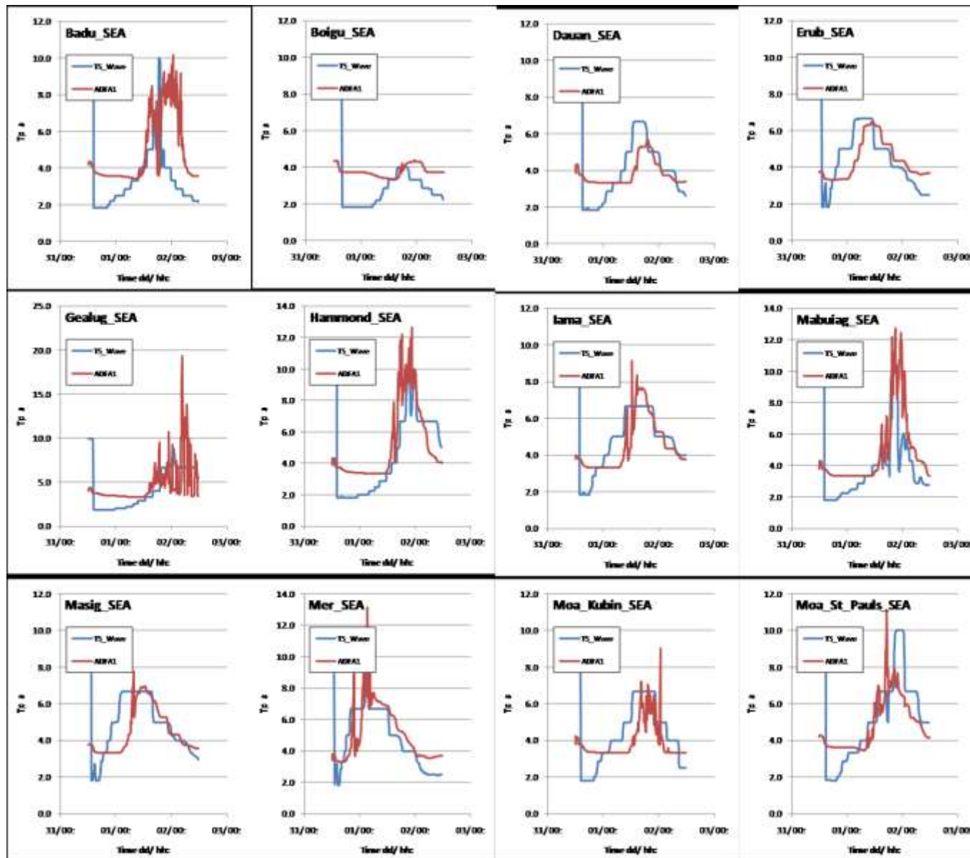
Figure L-3d Example E-W Category 4 TC through Centre (Tp time series comparisons)
