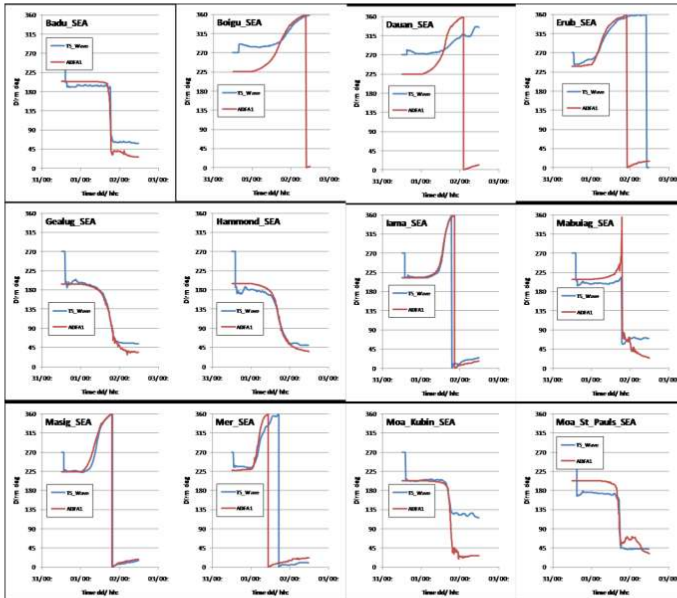
Figure L-3e Example E-W Category 4 TC through Centre (Mean Direction time series comparisons)
