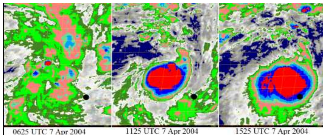
Figure 6-3 Enhanced infrared satellite imagery during the rapid intensification of an unnamed tropical cyclone near Fiji in April 2004. The green encloses areas with temperatures colder than -30^{\circ}\text{C} grading to -80^{\circ}\text{C} in the red areas (indicator of a cloud structure of an intense storm system).
