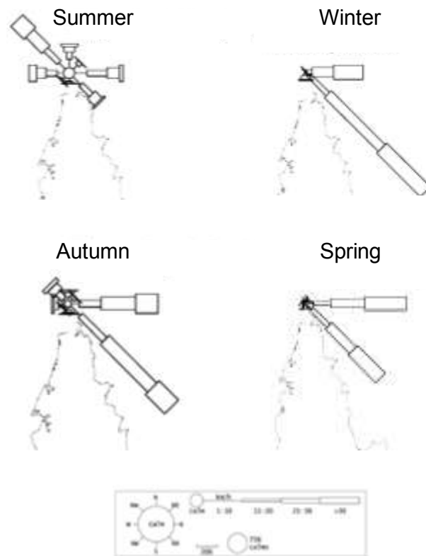
Figure 3-3 Thursdays Island mean wind speed roses (BoM analysis 1961-1990).
