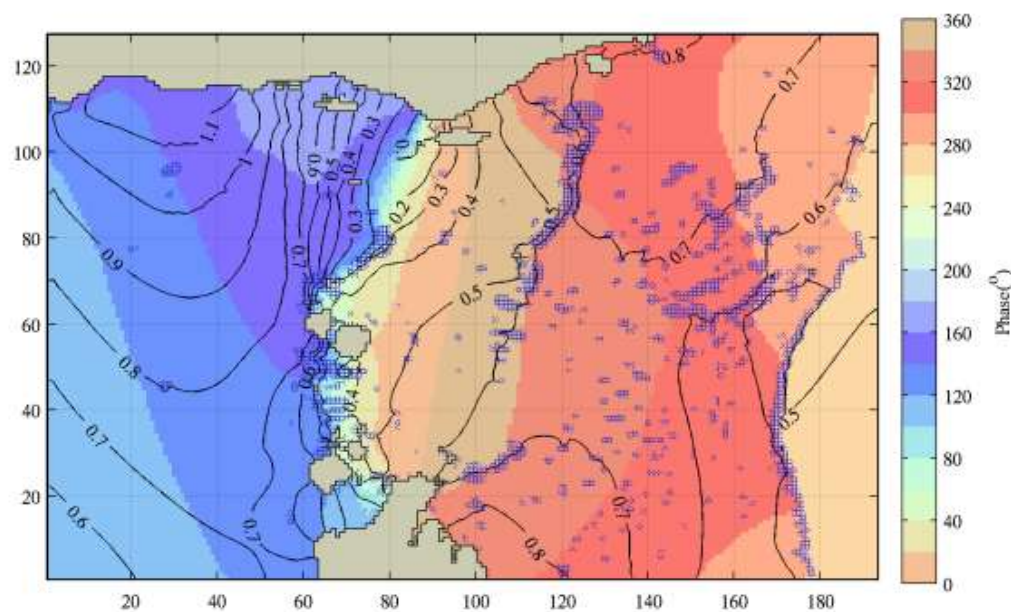
Figure 4-5 The TS-modelled M_2 component tidal propagation pattern.
